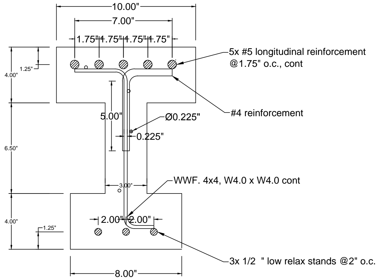
Cross Section
